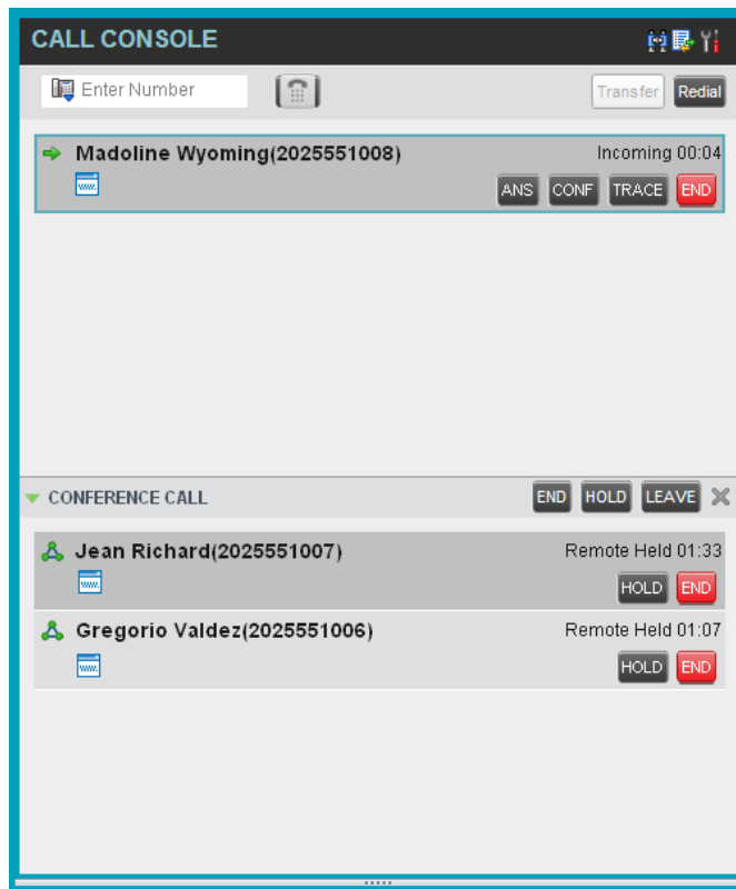
Call Console
