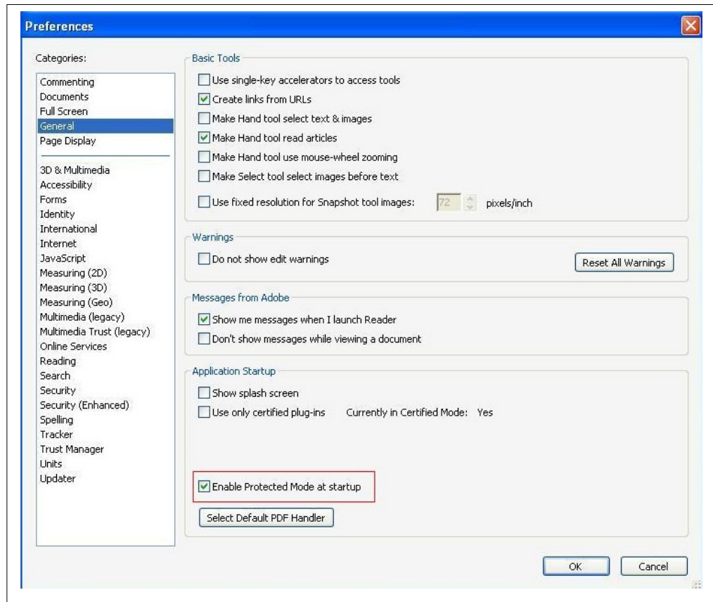
Preferences – General
